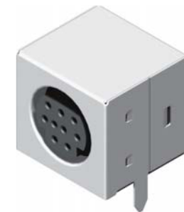
Part No.:MDJ-508H-9-L
