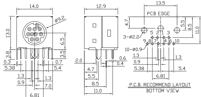
Part No.:MDJ-508H-10-L
