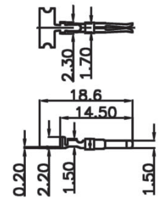
CRIMP TERMINAL
