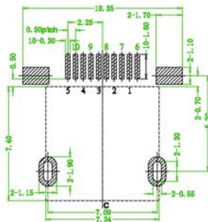
Recommended P.C.B Layout(Top Side) Tolerance=±0.05
