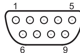
Pic. 6 Sub-D male connector
