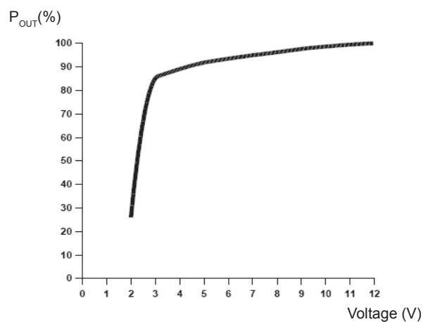
Pic. 4 Rel. optical power output vs.driver voltage
